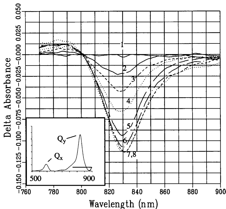
FIGURE 3 Difference spectra obtained upon 600 nm Q_x excitation of B820 antenna subunits at 600 nm. Shown is the in-growth of the signal. Spectra were taken at t = -300 , 100, 233, 267, 500, 633, and 767 fs; and 7.4 ps (.....), respectively. Compared with Fig. 1, it is striking that the isosbestic point hardly shifts as a function of time. As in Fig. 1, the inset shows the absorption spectrum of the sample, with indication of the Q_x and Q_y absorption bands, as well as the region of the detection wavelengths (horizontal bar).
