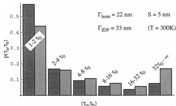
FIGURE 7 Distribution of transfer times in an inhomogeneously broadened LHA, directly after nonselective excitation (left) and after equilibration (right). Parameters are taken from the case \kappa = 0.7 in Table 1. Each bar represents a range (\tau_a, \tau_b) of times in units of \tau_0 . The height of the bar gives the probability p(\tau_a, \tau_b) that a transfer time is in this range. It is obvious that after equilibration, slower transfer times become more prominent; however, more than 50% of the transfer times is still faster than 4 \tau_0 , corresponding to 400–600 fs.
