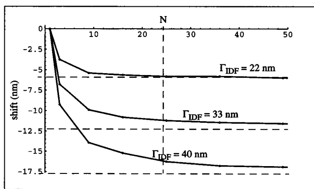
FIGURE 6 Equilibration shift of the average of the excitation energy distribution for systems with a finite number of subunits ( N ) for \Gamma_{IDF} = 22, 33 , and 40 nm ( \kappa = 1.4, 0.7 , and 0 respectively). Calculations were done for T = 300 K, which corresponds to k_B T = 16 nm in the LH1 absorption band (at 880 nm). It is obvious that the thermal distribution over 25 subunits closely resembles the thermal distribution over an infinitely large number of connected subunit (---) for \Gamma_{IDF} = 33 nm. As expected: for larger inhomogeneous widths (larger \Gamma_{IDF} ), a larger number of subunits in a system is needed to make the thermal distribution over the system similar to the distribution in an infinite system.
